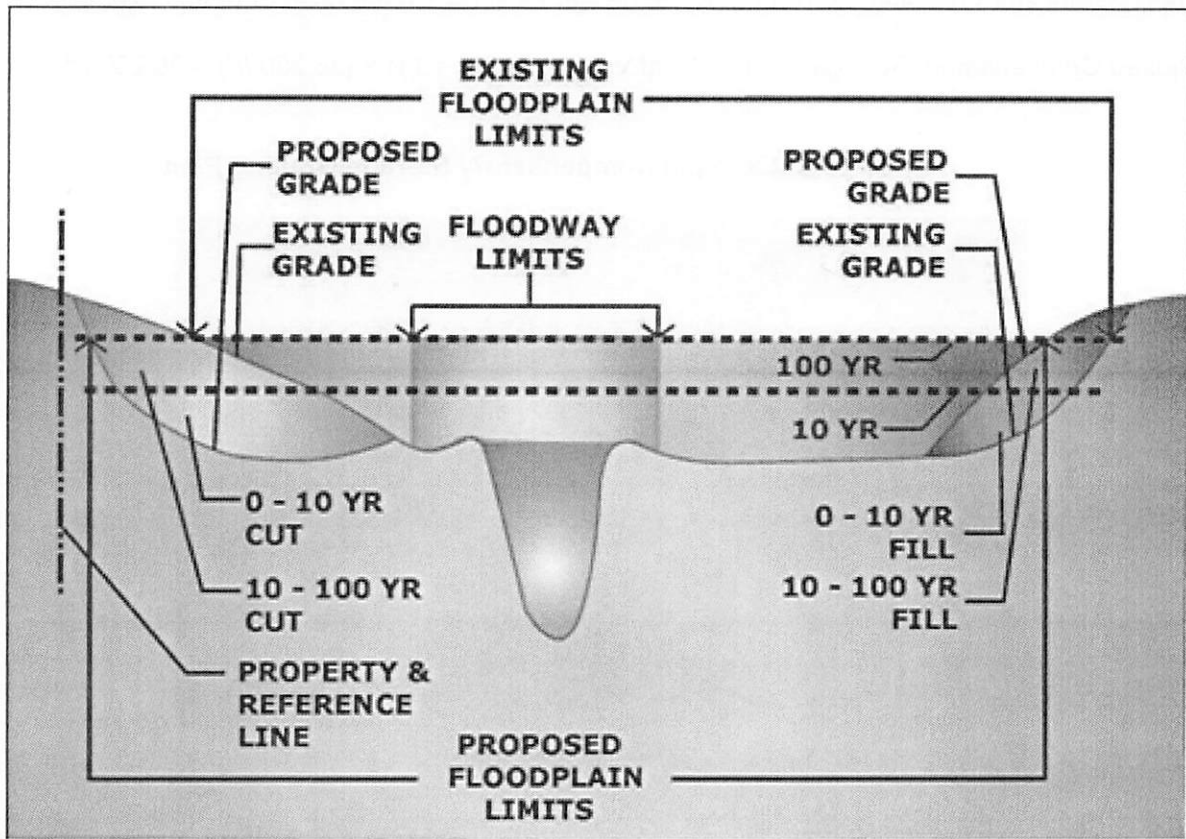
Figure 10-4 – Example Cross Section D-D
