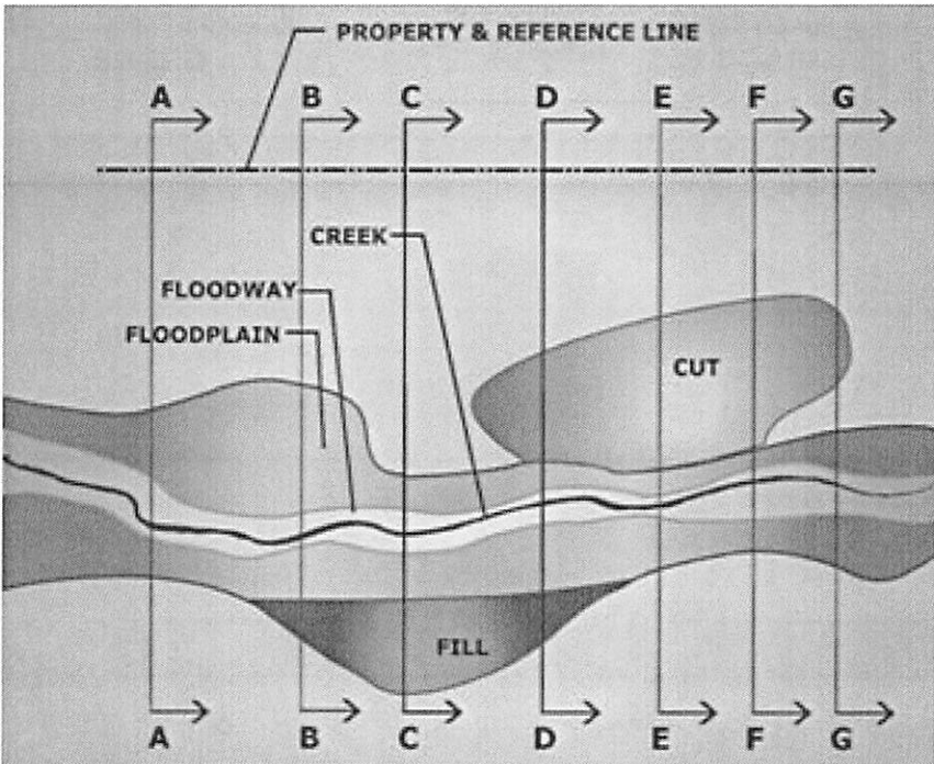
Figure 10-3- Example Compensatory Storage Grading Plan
