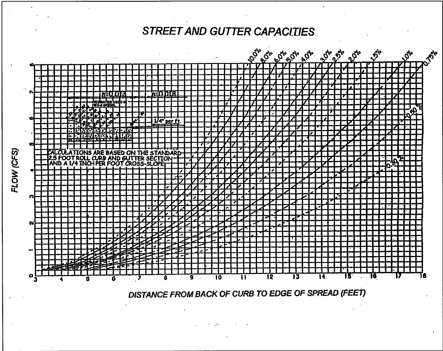
FIGURE 4-1 Street and Gutter Capacities (continuous grade)
