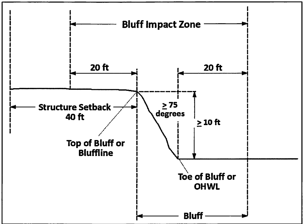
Figure 10-2 Natural Escarpment Bluff and Bluff Impact Zone
