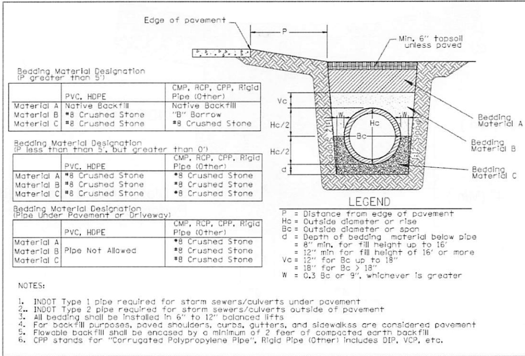
FIGURE 4-2 Bedding and Backfill Standards for Storm Sewers
