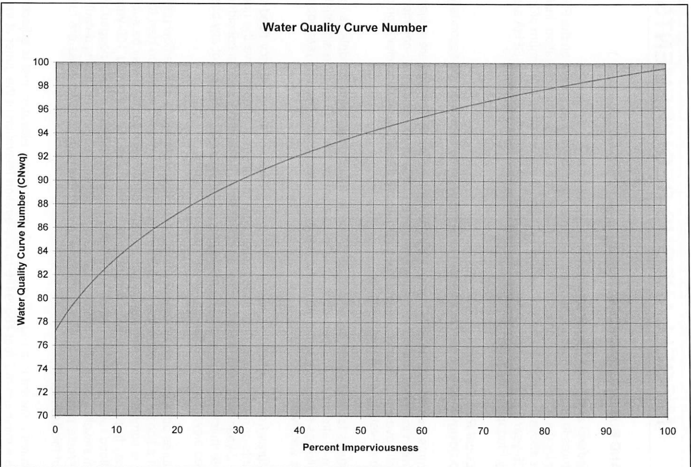
Figure 9-1 Curve Number Calculation for Water Quality Storm Event
