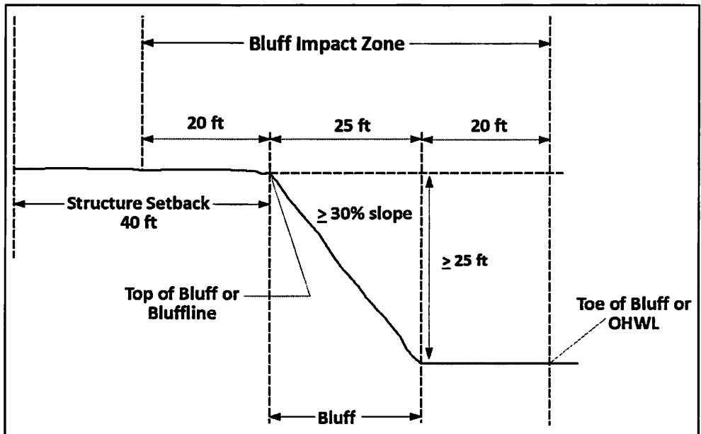
Figure 10-1 Bluff and Bluff Impact Zone
