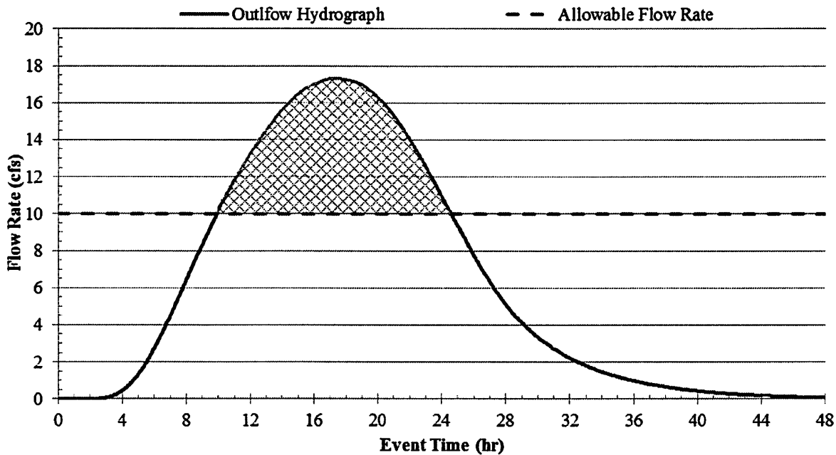
FIGURE 3-1 Required Storage Volume Determination Example
